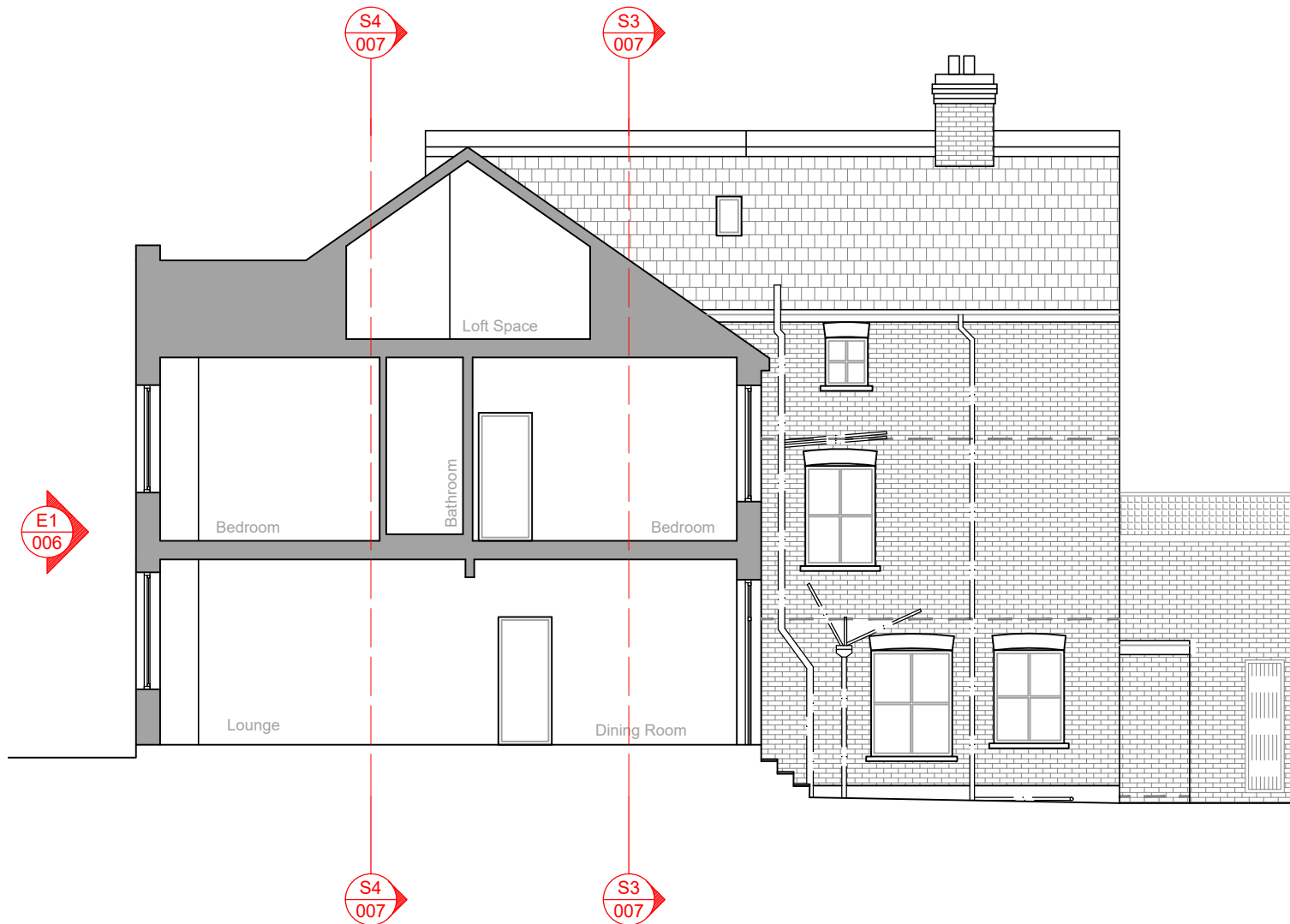
01 Existing Section S1 1:100 @ A3
