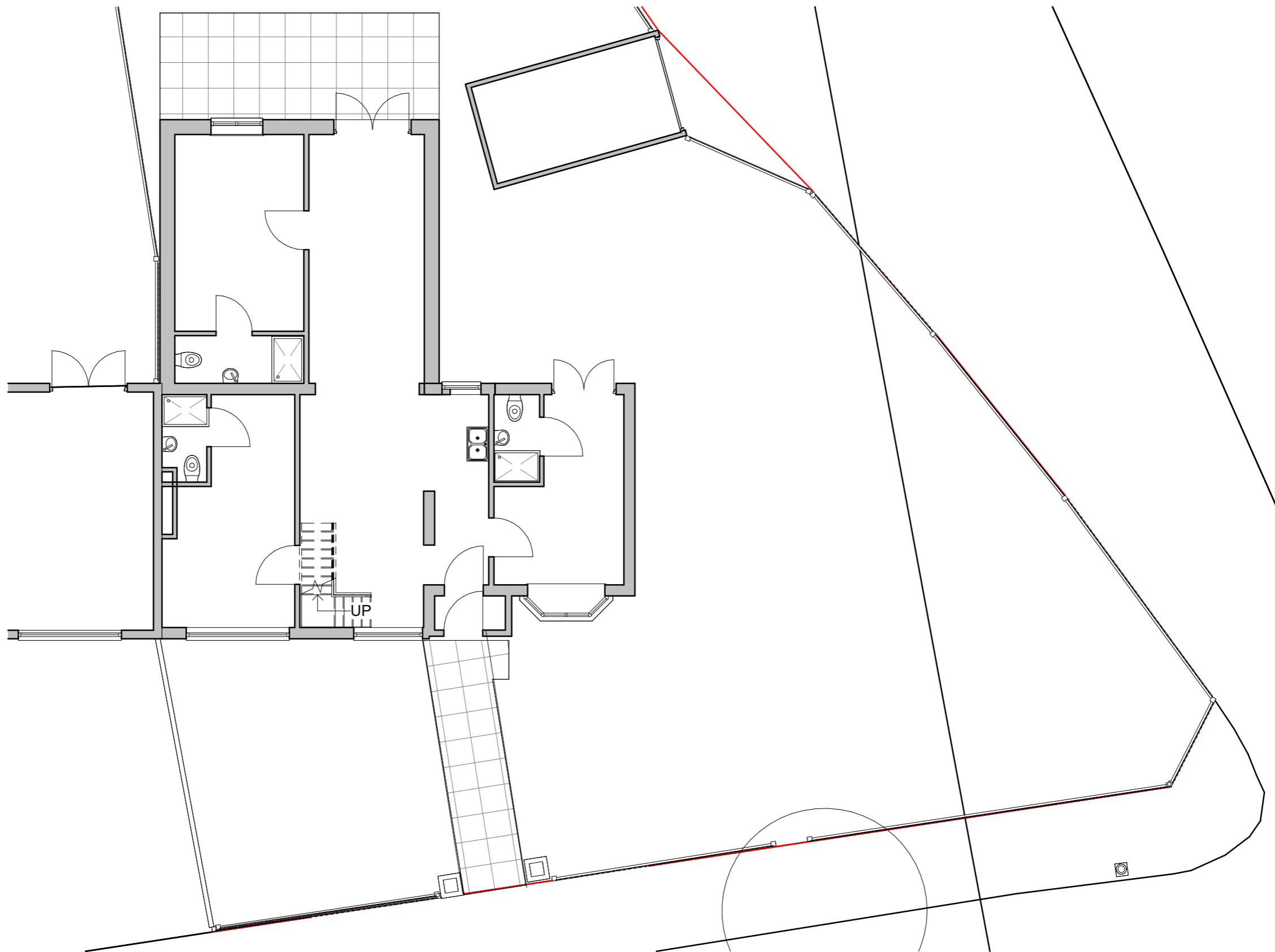
① Ground Floor 1 : 100
