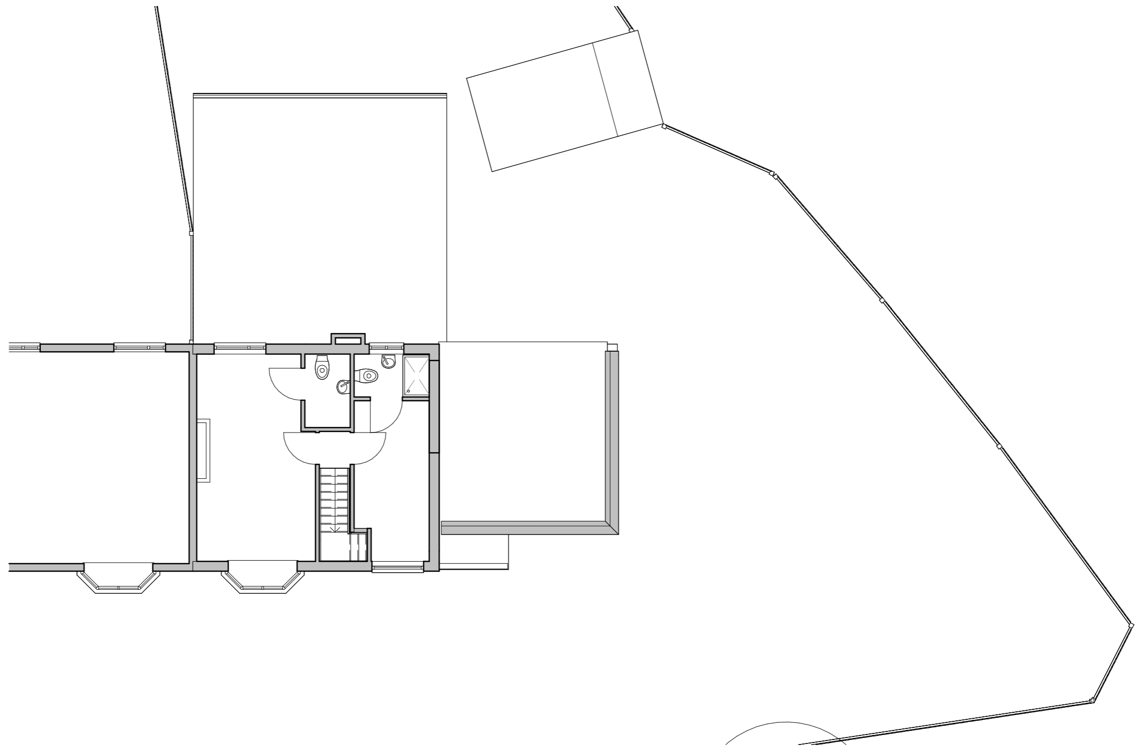
① First Floor 1 : 100
