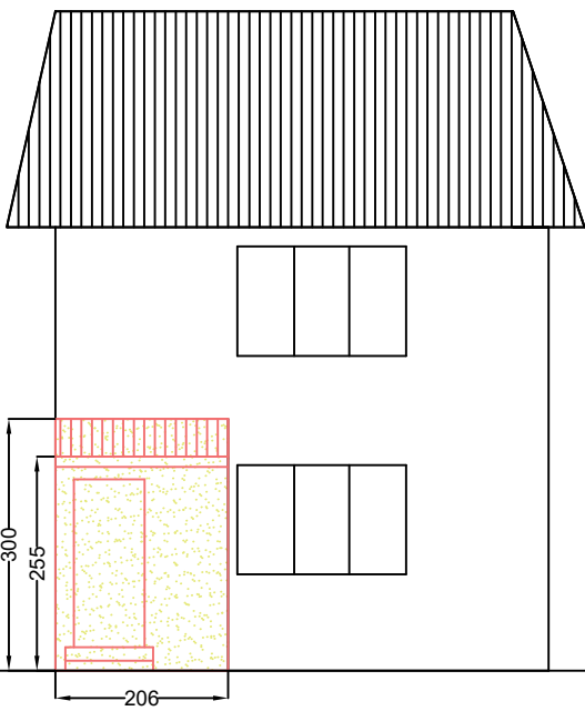
Front elevation- south
