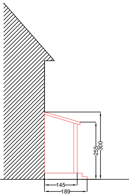
Side elevation - east
