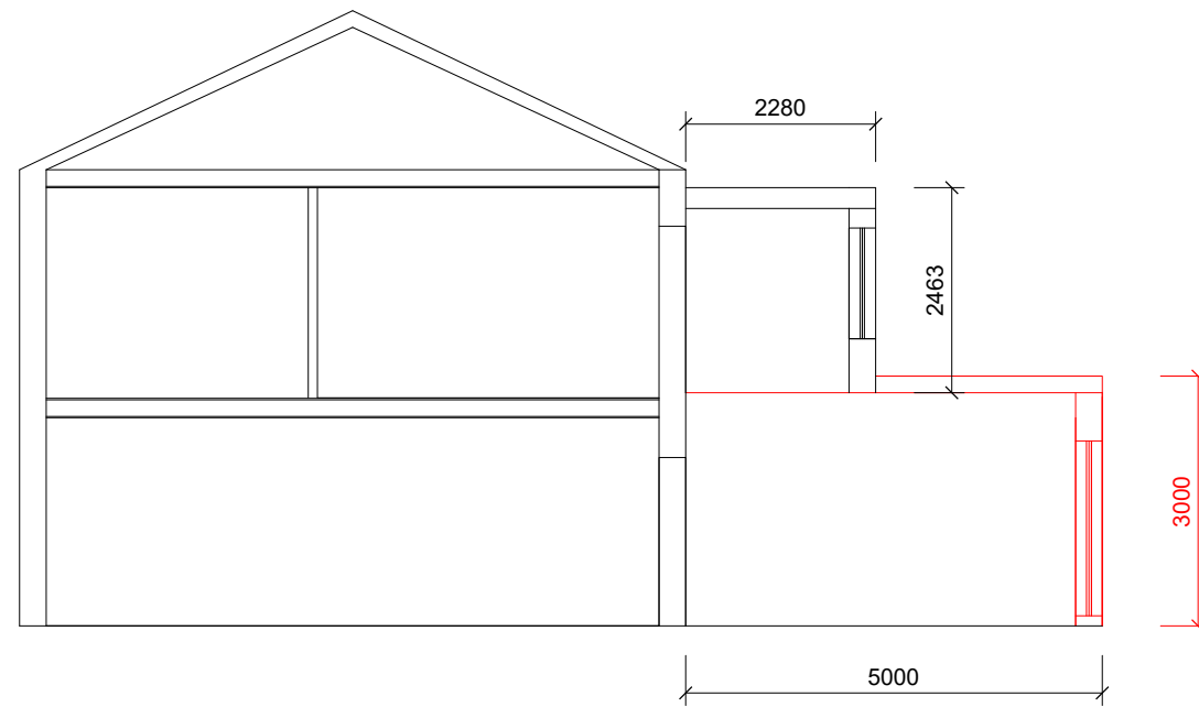
PROPOSED SECTION
