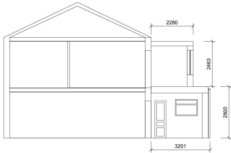
EXISTING SECTION
