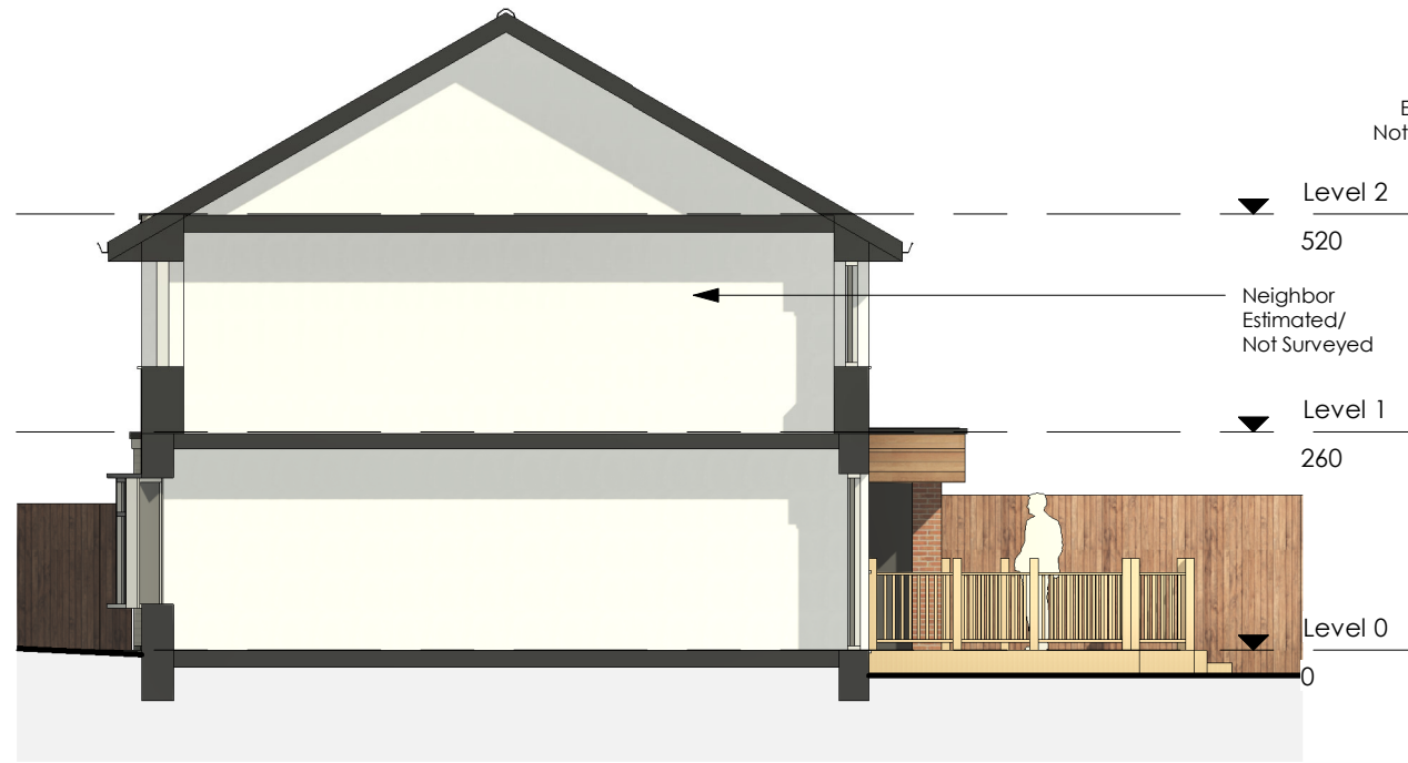
Existing R Side 1:100
