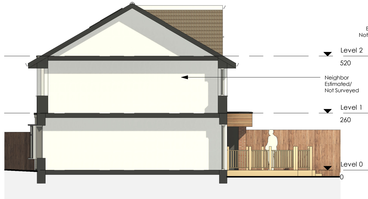
Proposed R Side 1:100
