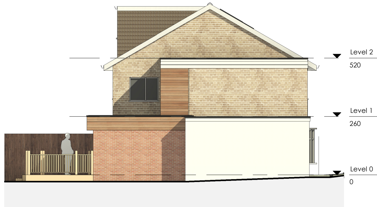
Proposed L Side 1:100
