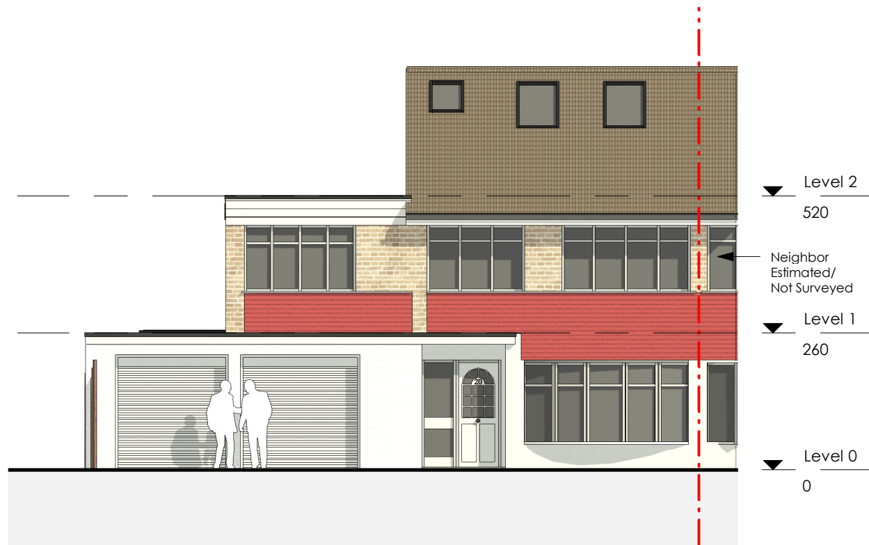
Proposed Rear 1:100
