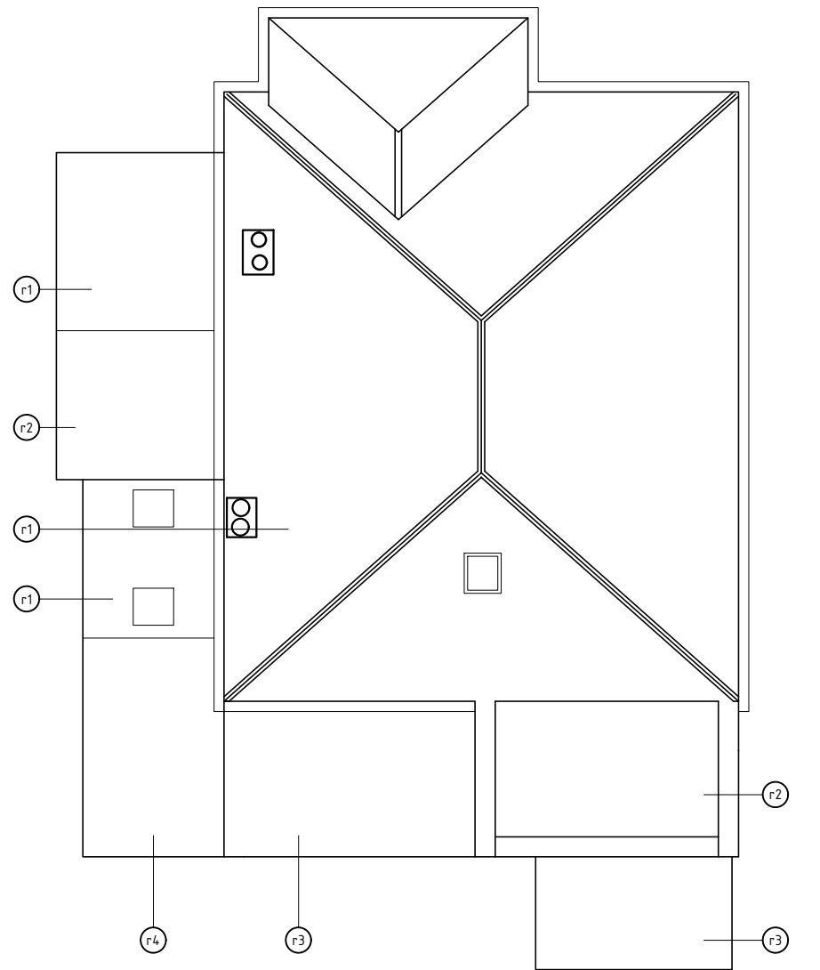
Existing roof plan 1:100 2m 0 2m 4m 6m 8m 10m
