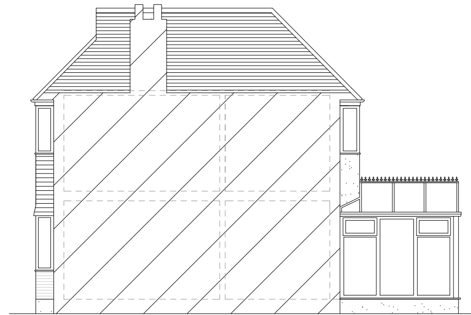
Side (N/E) Elevation Existing
