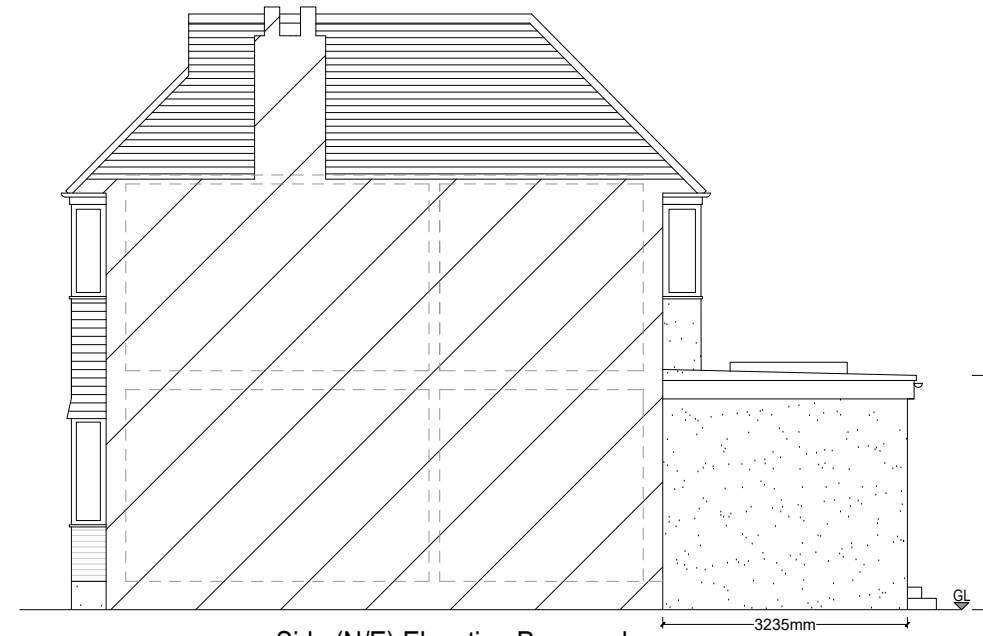
Side (N/E) Elevation Proposed
