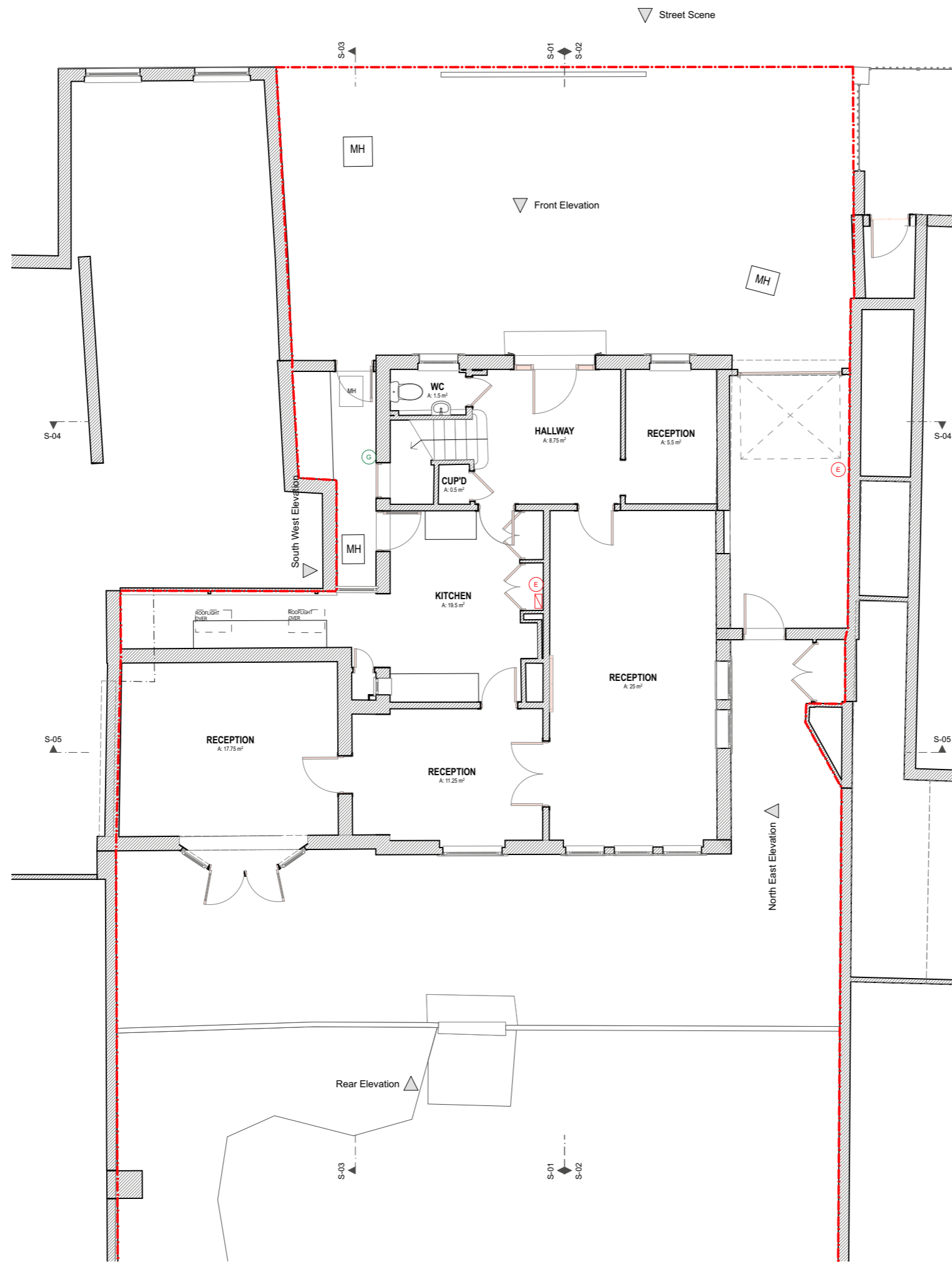
Ground Floor 1:100
