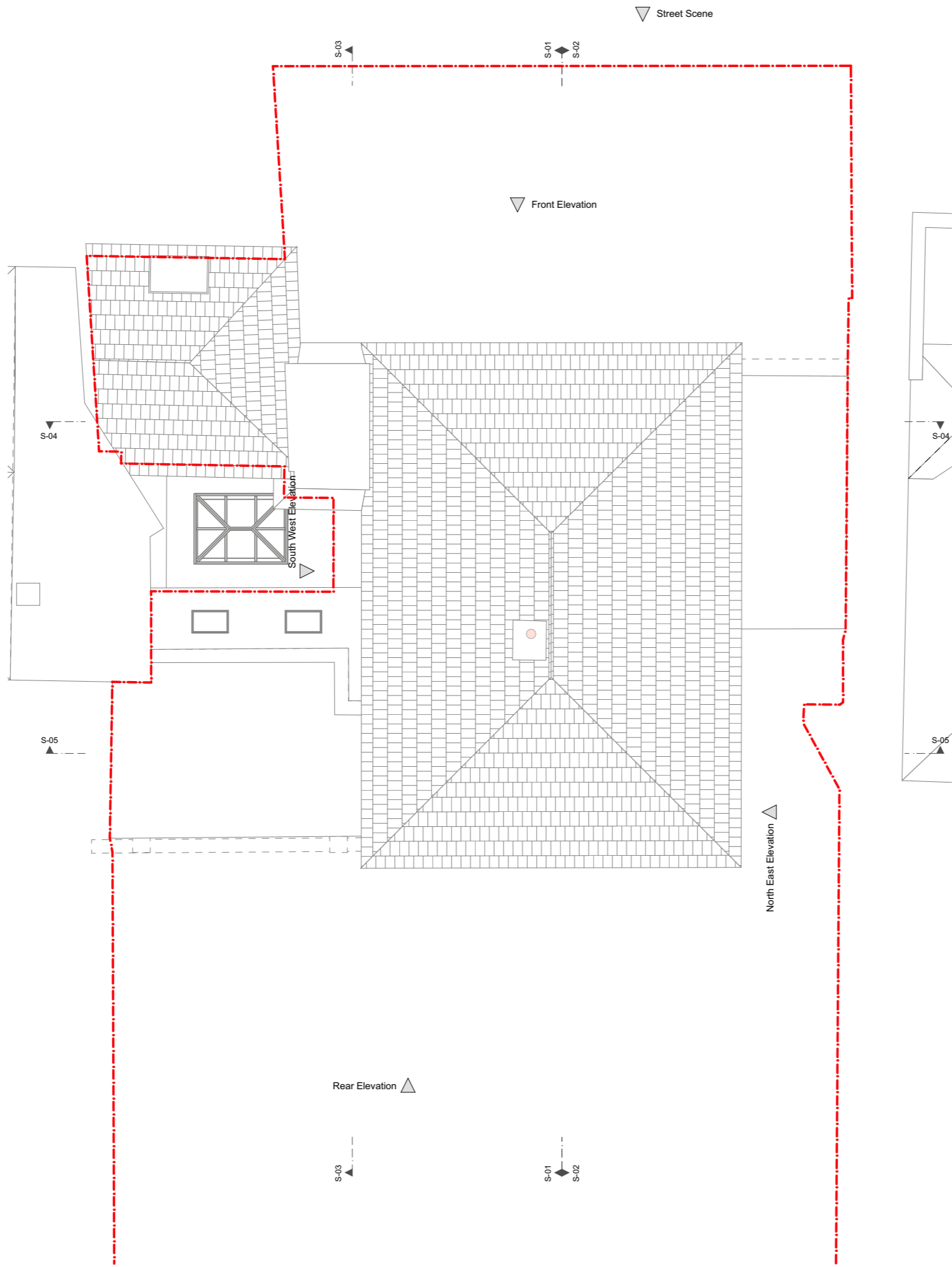
Roof Plan
