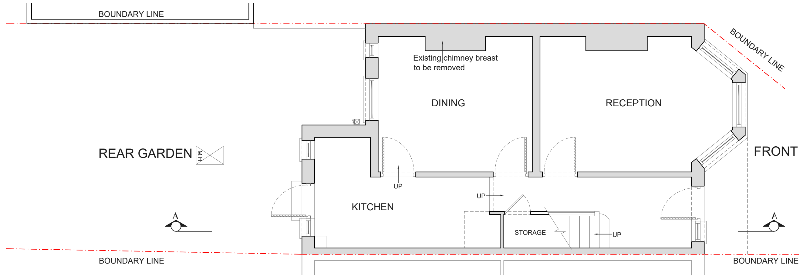
EXISTING GROUND FLOOR PLAN SCALE 1:50
