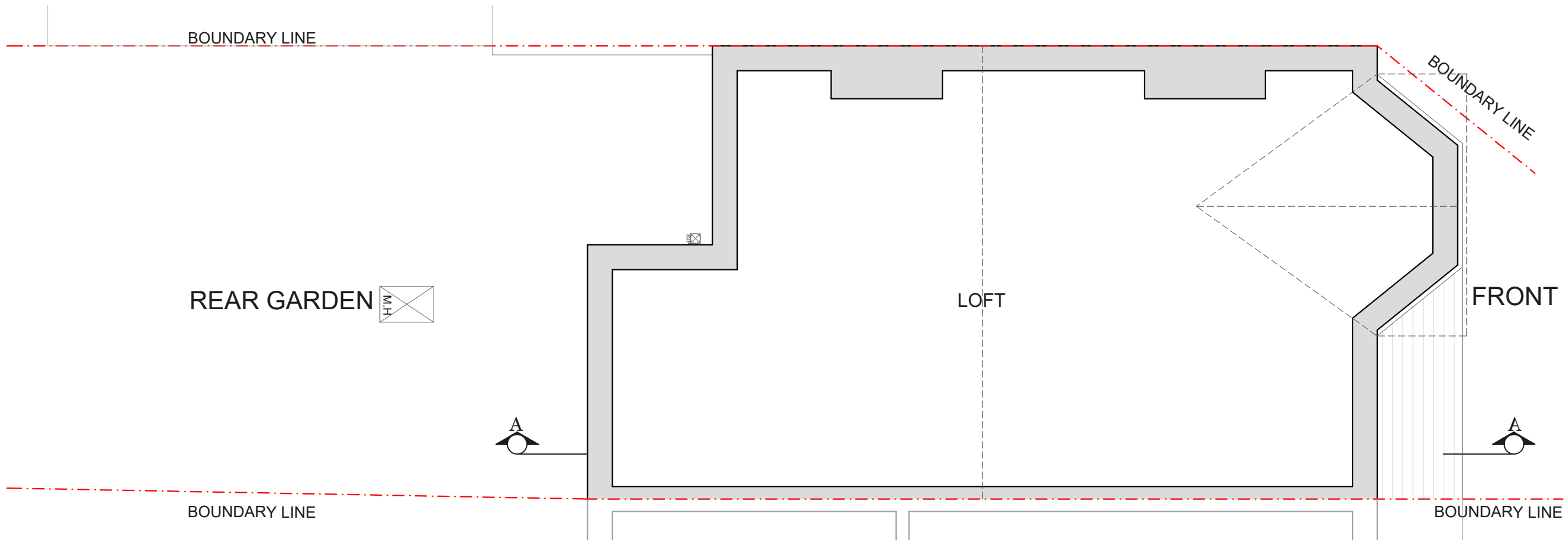
EXISTING LOFT FLOOR PLAN SCALE 1:50
