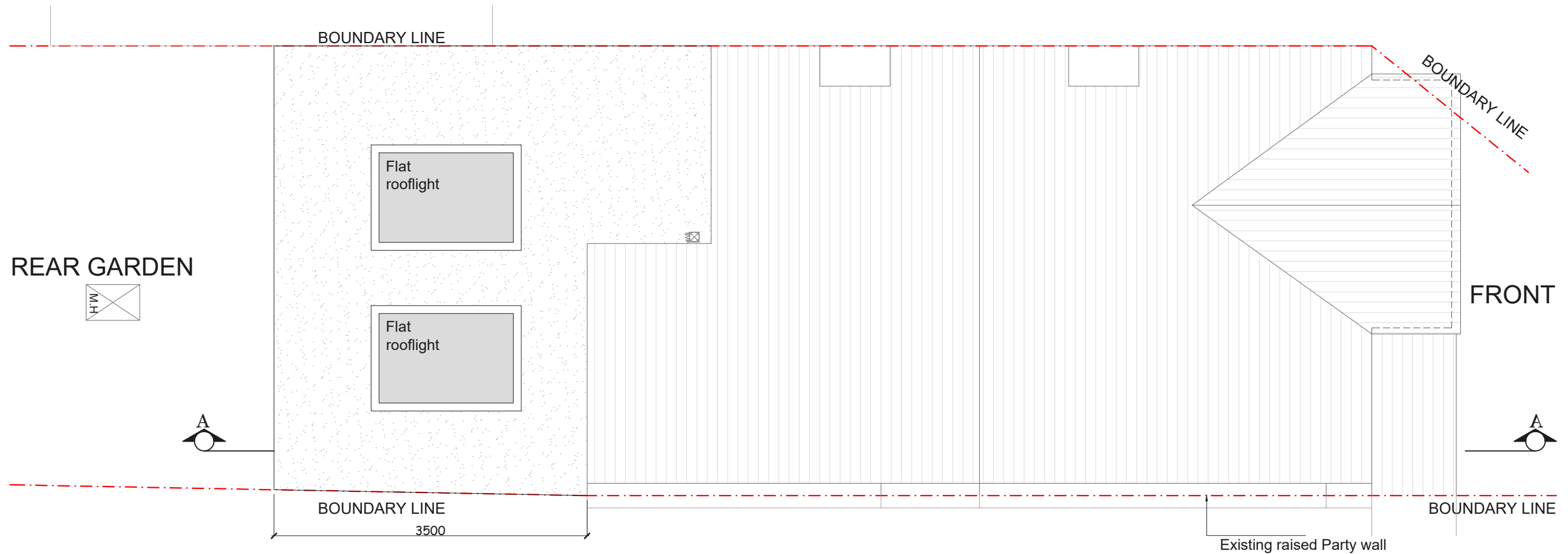
PROPOSED ROOFTOP PLAN SCALE 1:50
