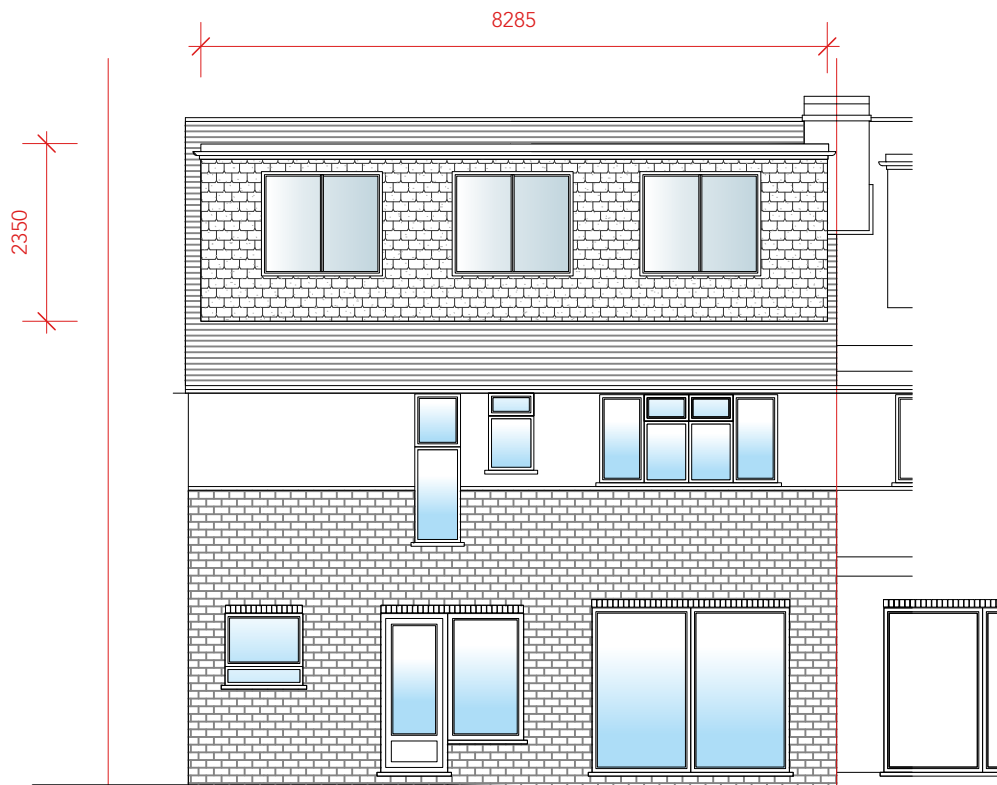
Rear Elevation C
