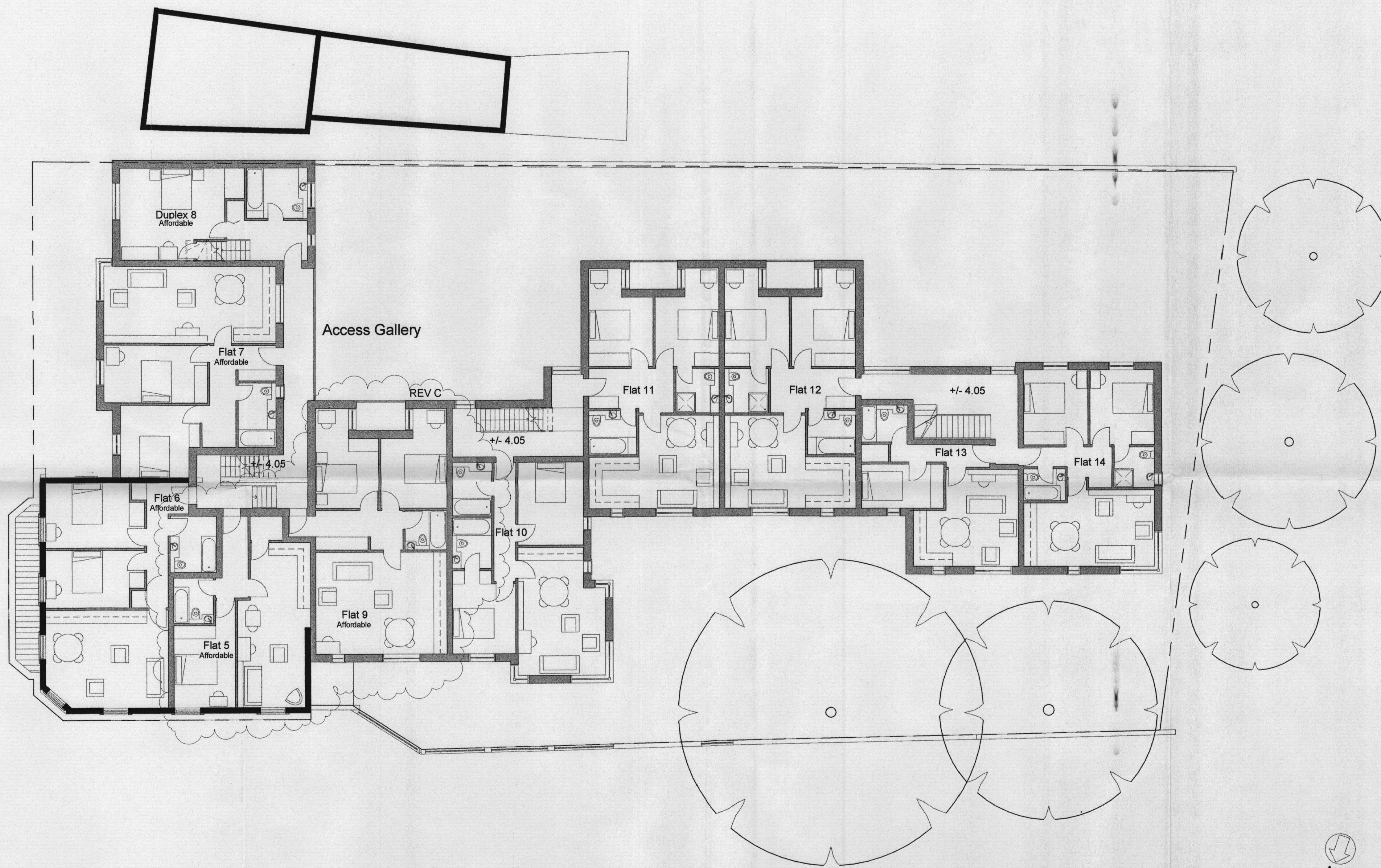
1 Proposed First Floor 1:100 @ A1 1:200 @ A3
