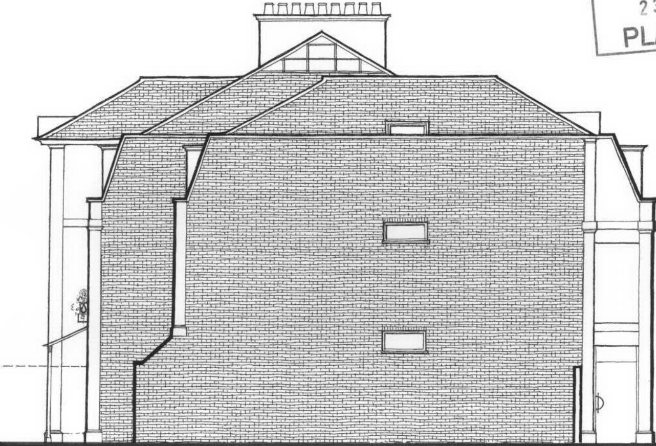
EAST ELEVATION
