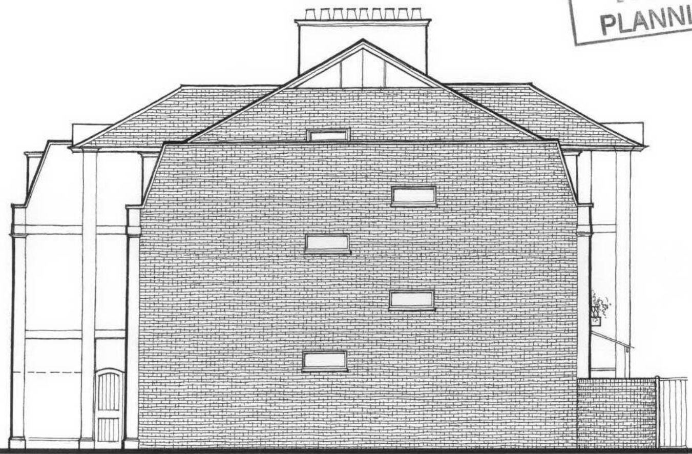
WEST ELEVATION
