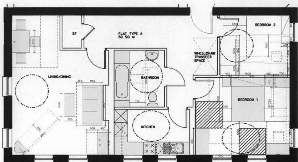
FLAT TYPE A - FIRST FLOOR
