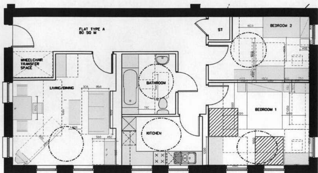
FLAT TYPE A - GROUND FLOOR
