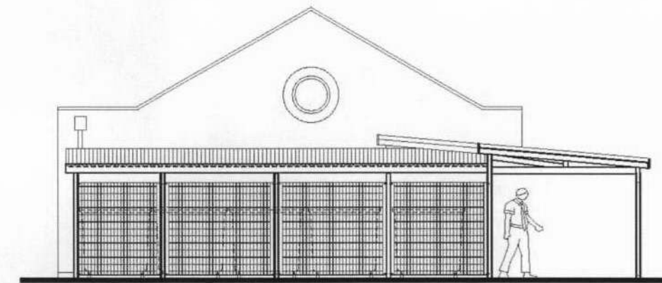
SOUTH ELEVATION
