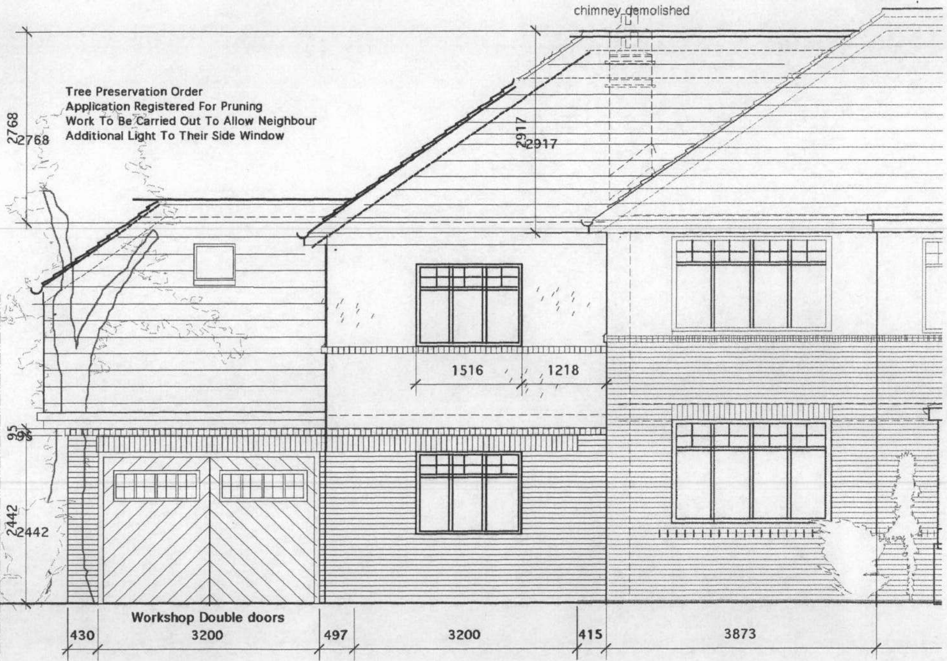
Front Elevation 1:50
