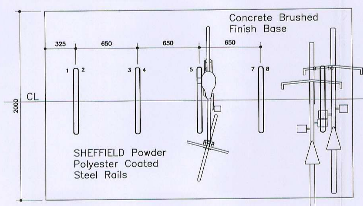
CYCLE PARKING LAYOUT
