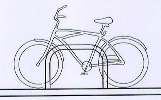
SHEFFIELD Powder Polyester Coated Steel Rails At 600 mm c/c
