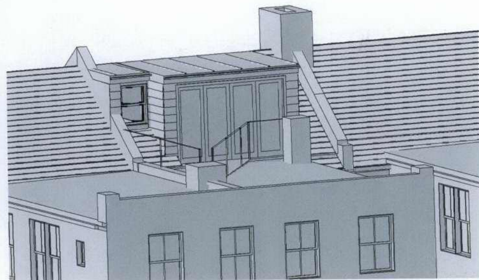
AXONOMETRIC VIEW OF NEW DORMERS FROM LEFT HAND SIDE, SECOND FLOOR LEVEL.
