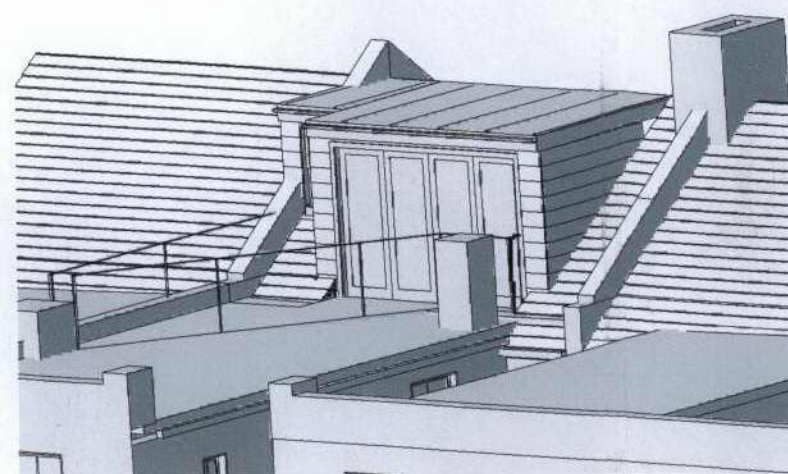
AXONOMETRIC VIEW OF NEW DORMERS FROM RIGHT HAND SIDE, SECOND FLOOR LEVEL.
