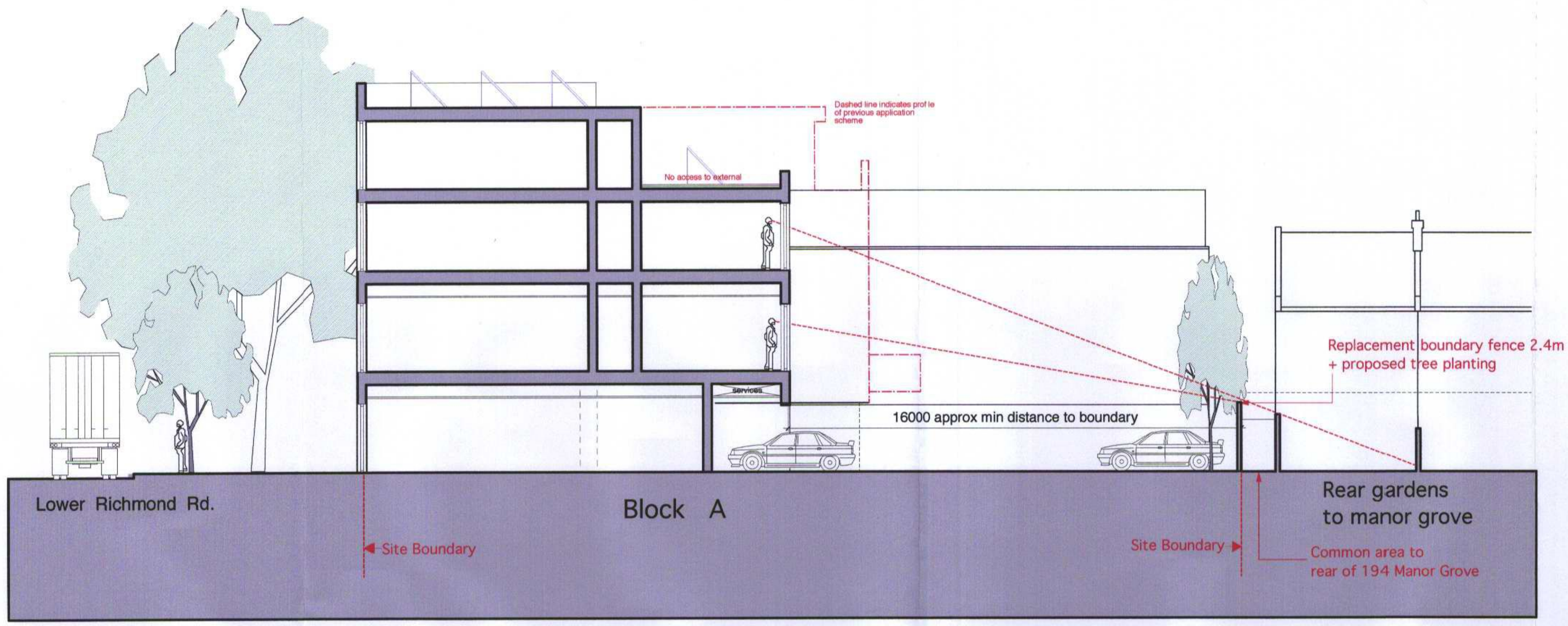
SECTION A-A THROUGH BLOCK A INDICATING POSSIBLE VIEWS TOWARDS 194 MANOR GROVE
