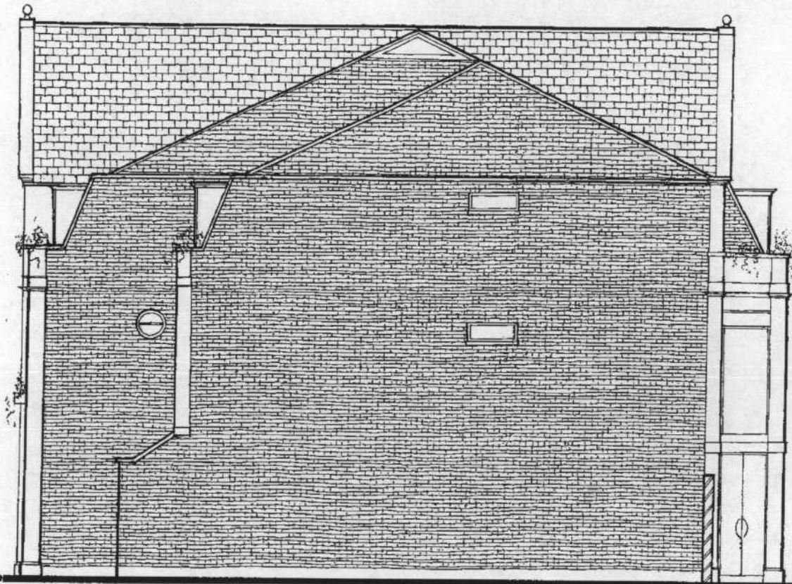
SIDE (NE) ELEVATION
