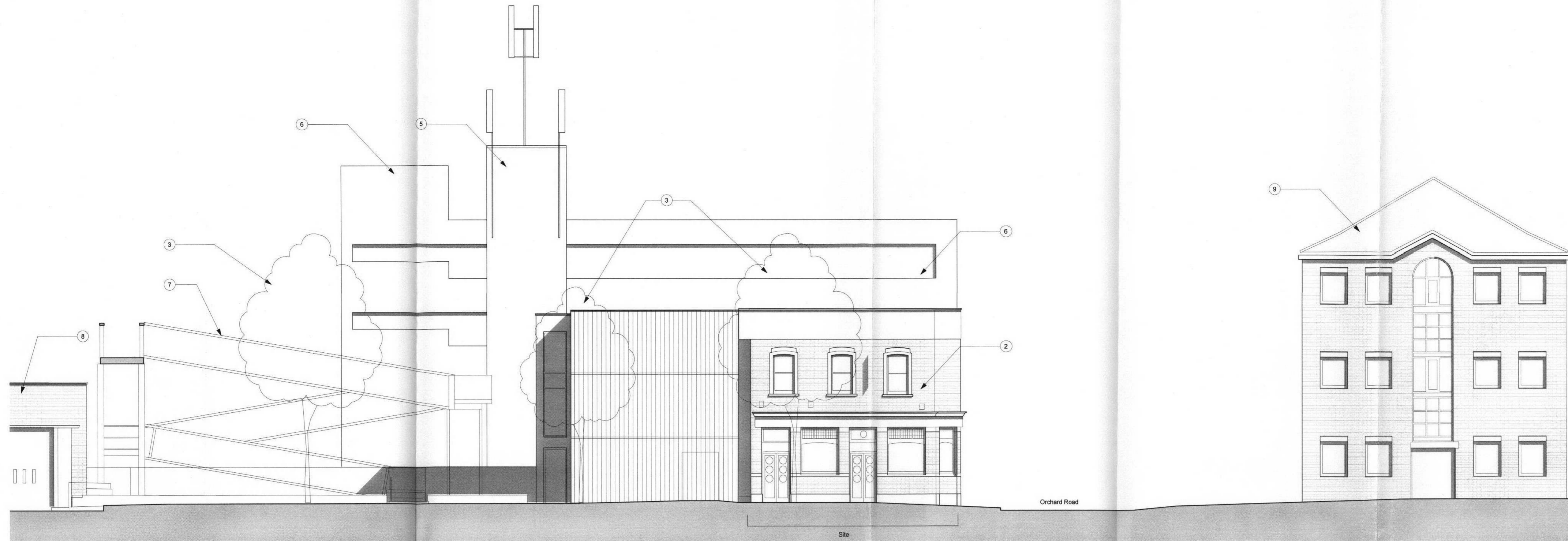
1 Existing Elevation - Lower Richmond Road EX(00)100 1:100
