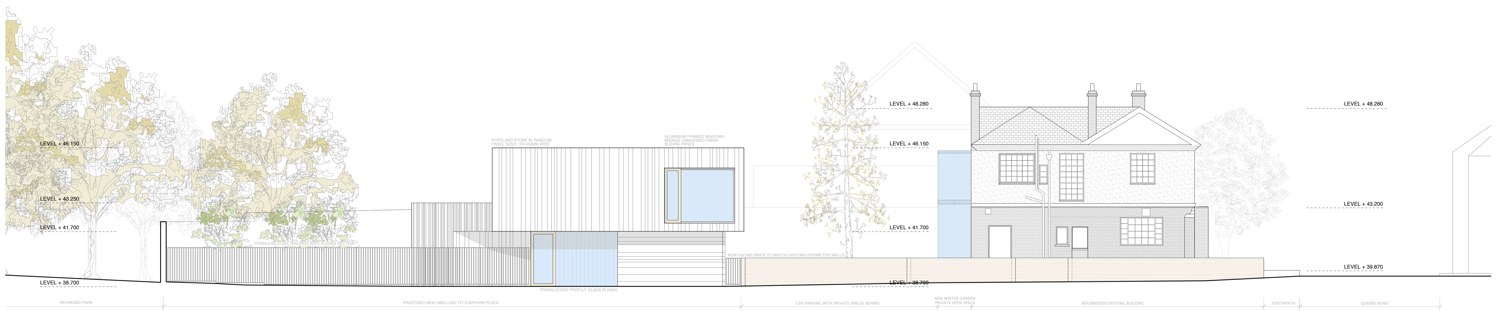
SECTION 2-2: ELEVATION TO STAFFORD PLACE 204 PROPOSED SITE SCALE 1:100
