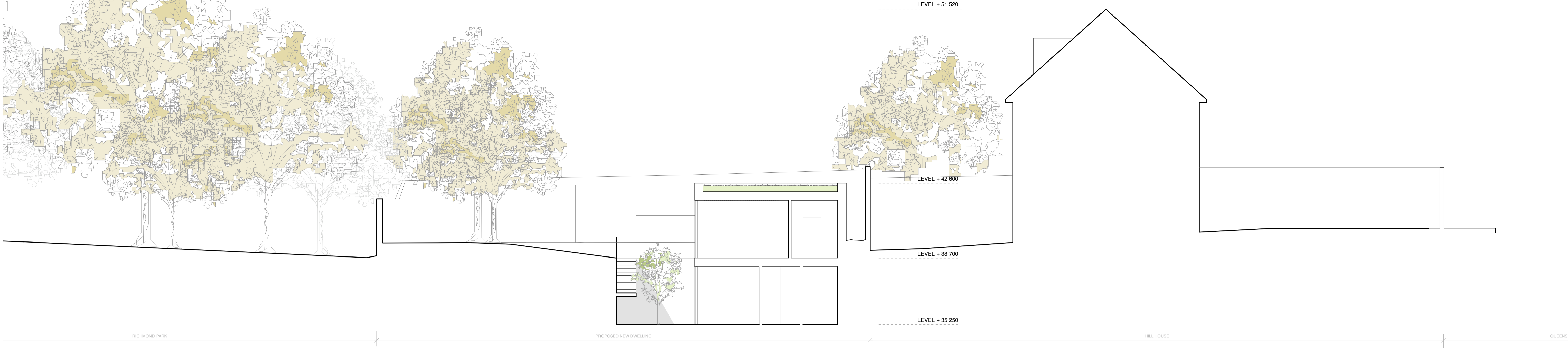
SECTION 7 206 PROPOSED SITE SCALE 1:100
