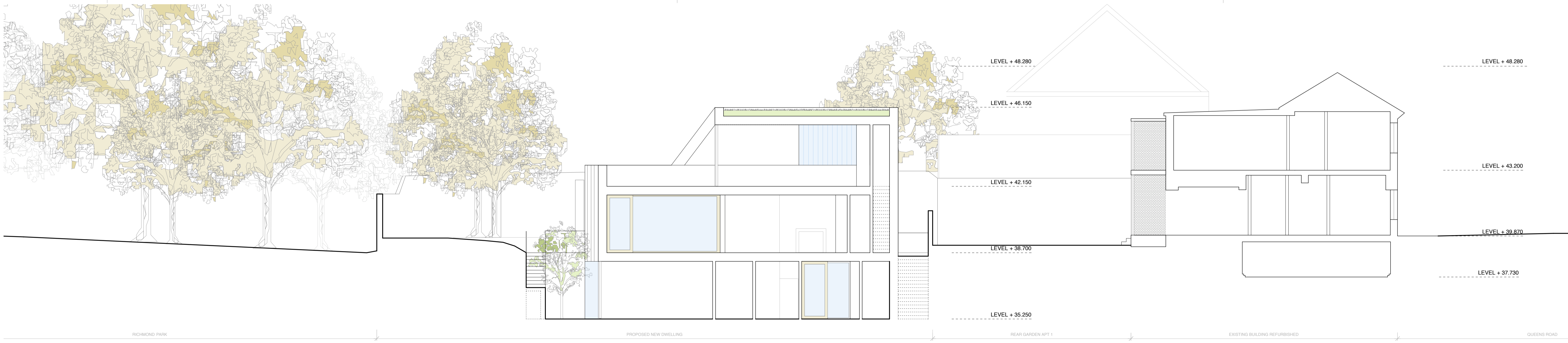
SECTION 9 206 PROPOSED SITE SCALE 1:100
