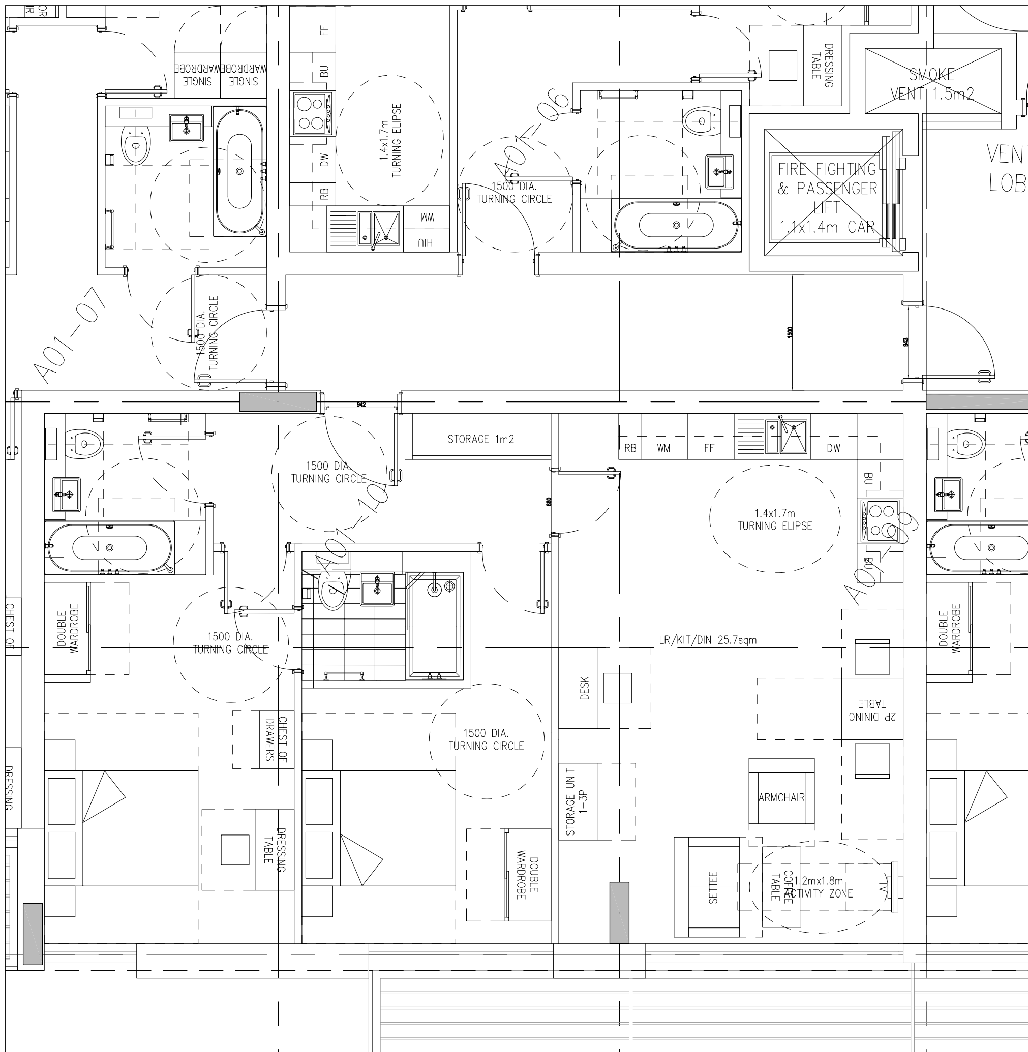
TYPICAL LAYOUT OF WHEELCHAIR USER COMPLIANT DWELLING
