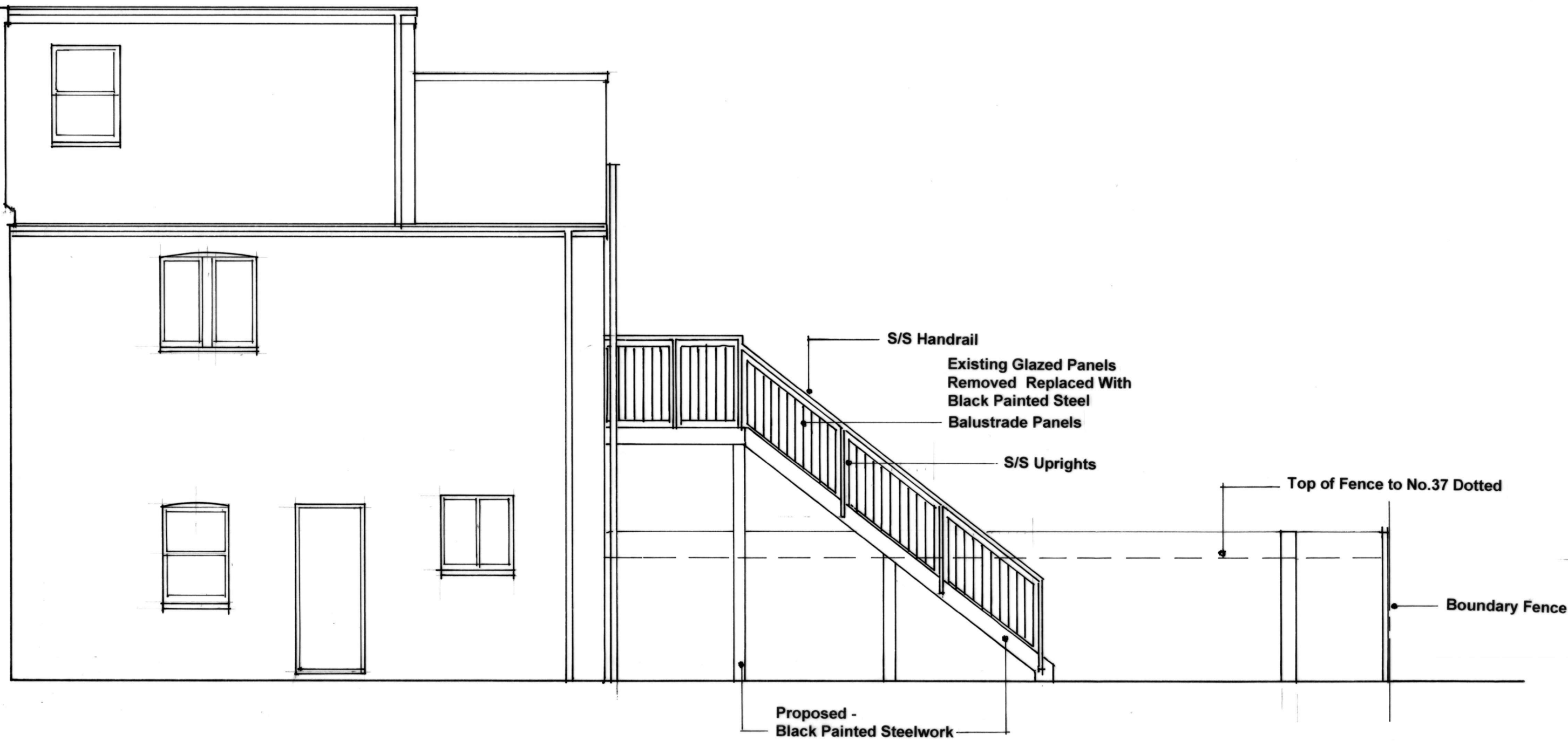
Side Elevation to No.37 (West) 1:50 at A3
