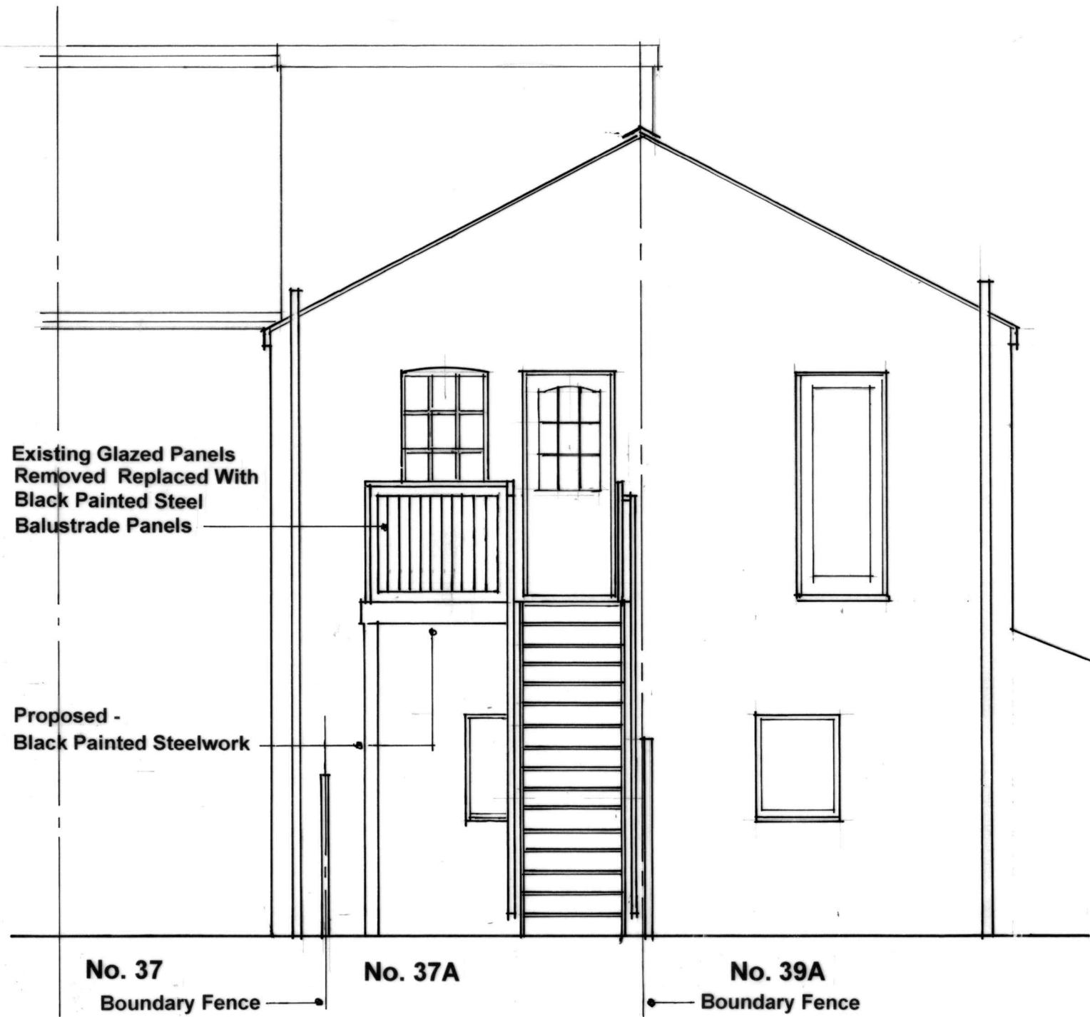
Rear Elevation 1:50 at A3
