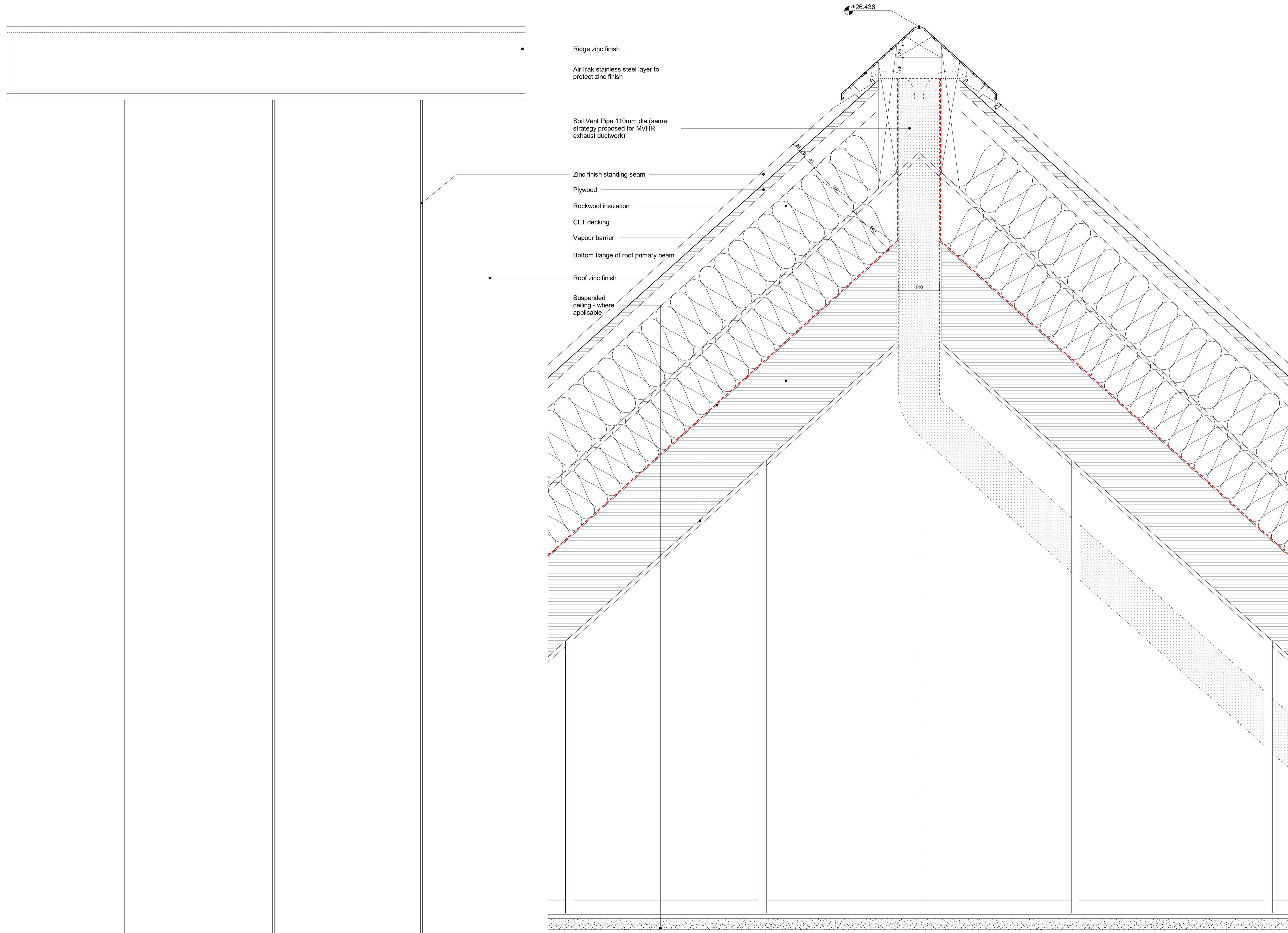
2 Roof ridge side elevation SK225 1:5
