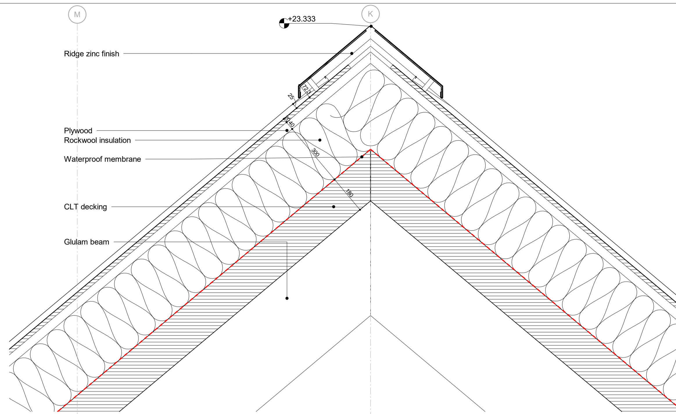
1 Roof Ridge Cross Section SK226 1:10
